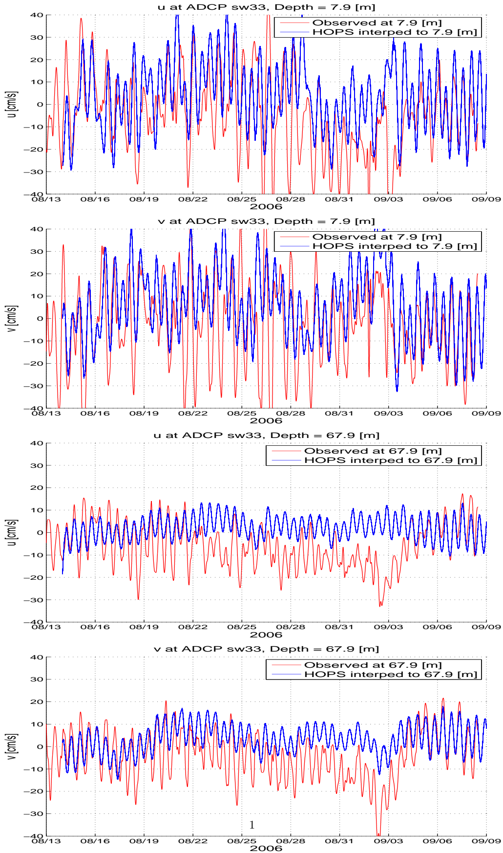
Figure 1. ADCP sw33, HOPS run in Jul10/PJH0/, (upper 2 panels): z7m, (bottom 2 panels): z67m.
