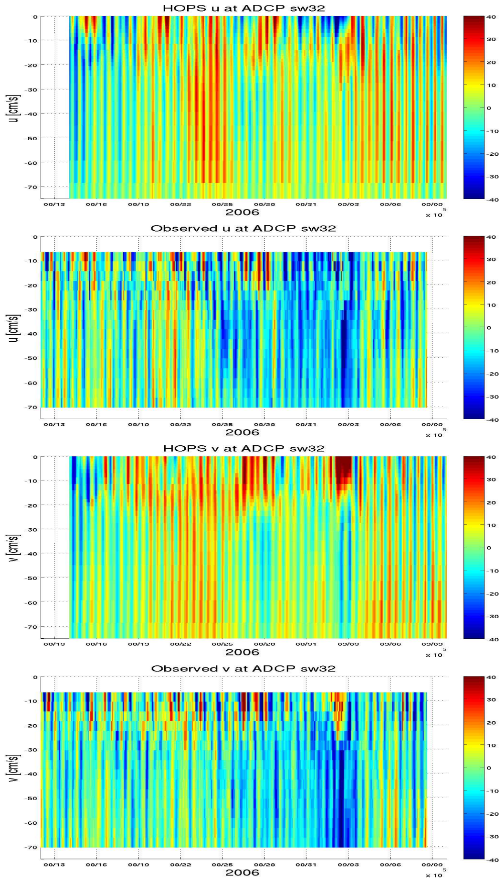
Figure 5. ADCP sw32, HOPS run in Jul10/PJH4/
