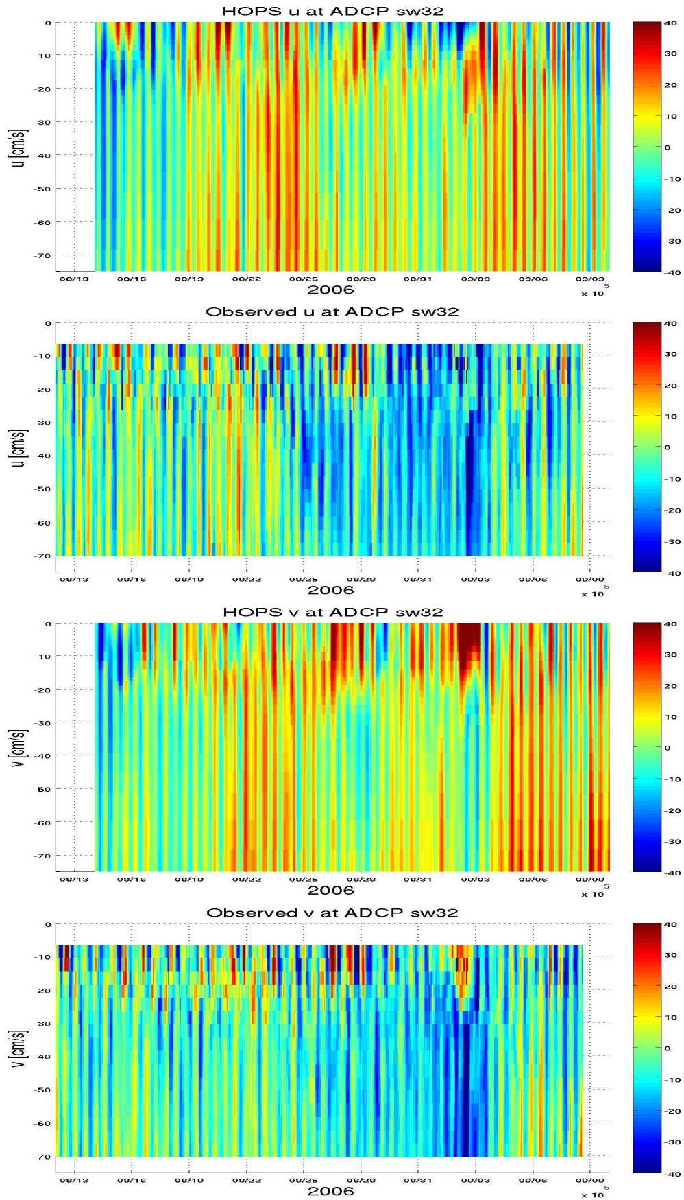
Figure 11. ADCP sw32, HOPS run in Jul10/PJH10/
