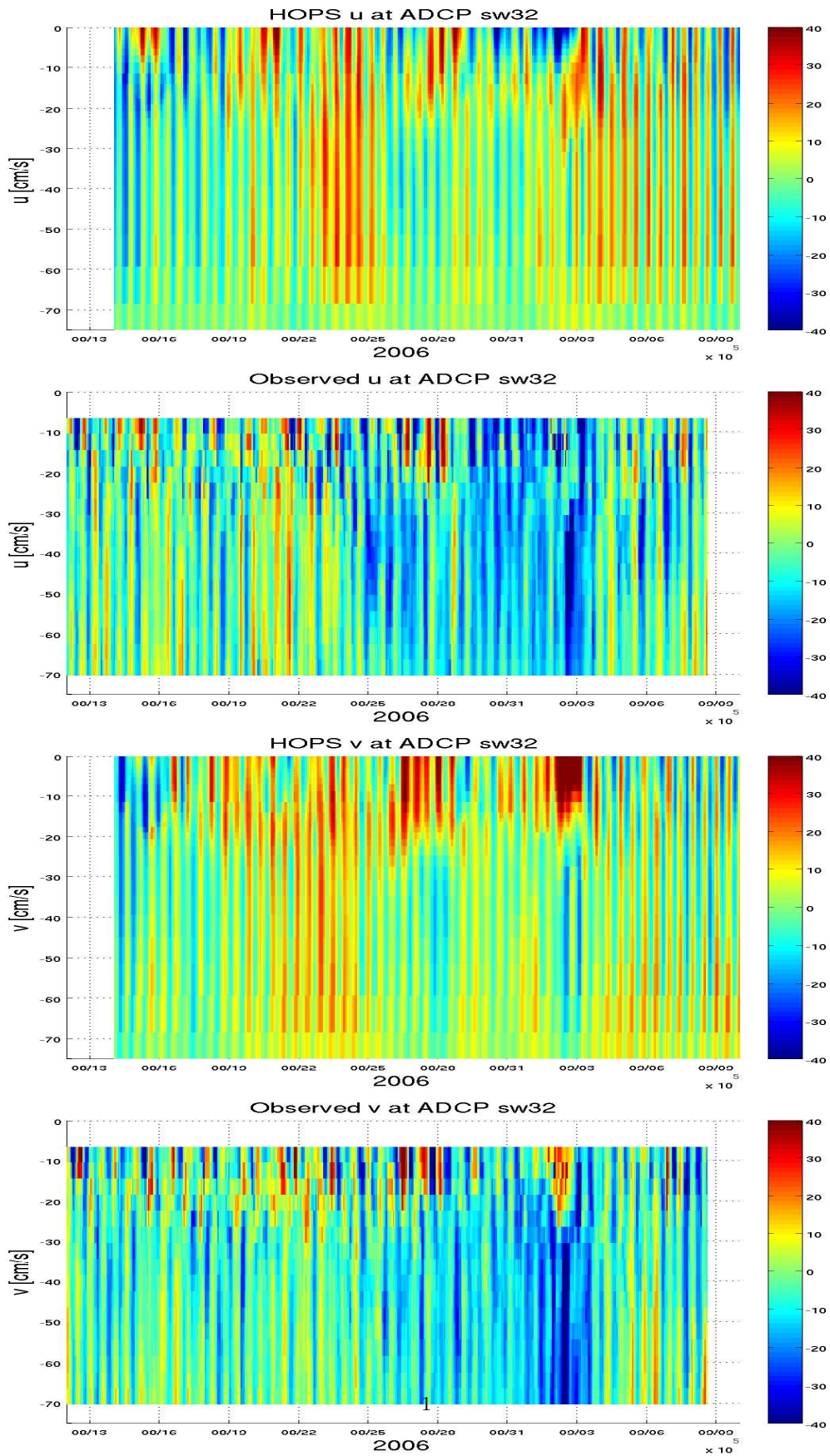
Figure 1. ADCP sw32, HOPS run in Jul10/PJH0/
