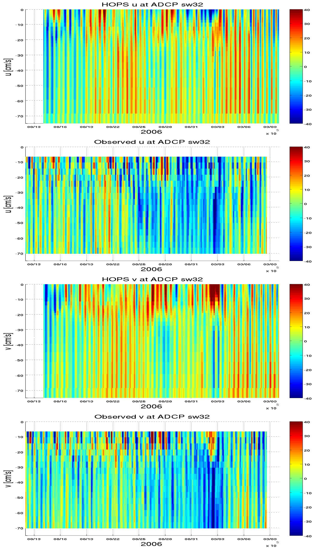
Figure 6. ADCP sw32, HOPS run in Jul10/PJH5/
