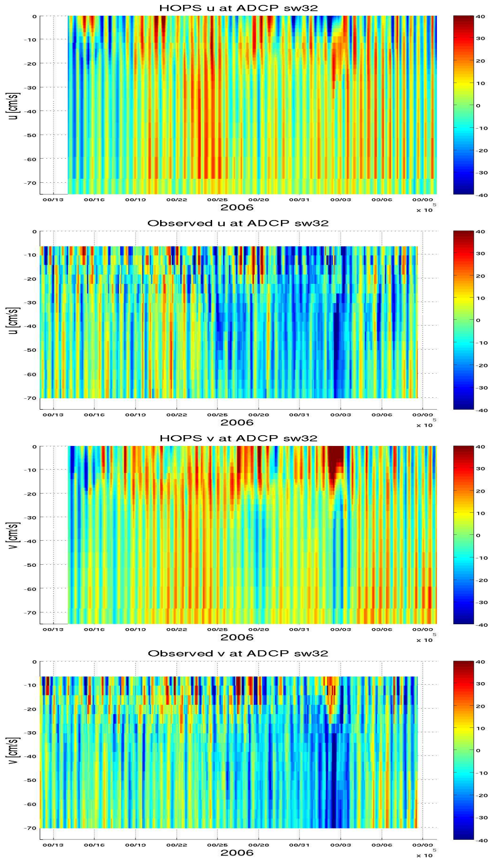
Figure 3. ADCP sw32, HOPS run in Jul10/PJH2/
