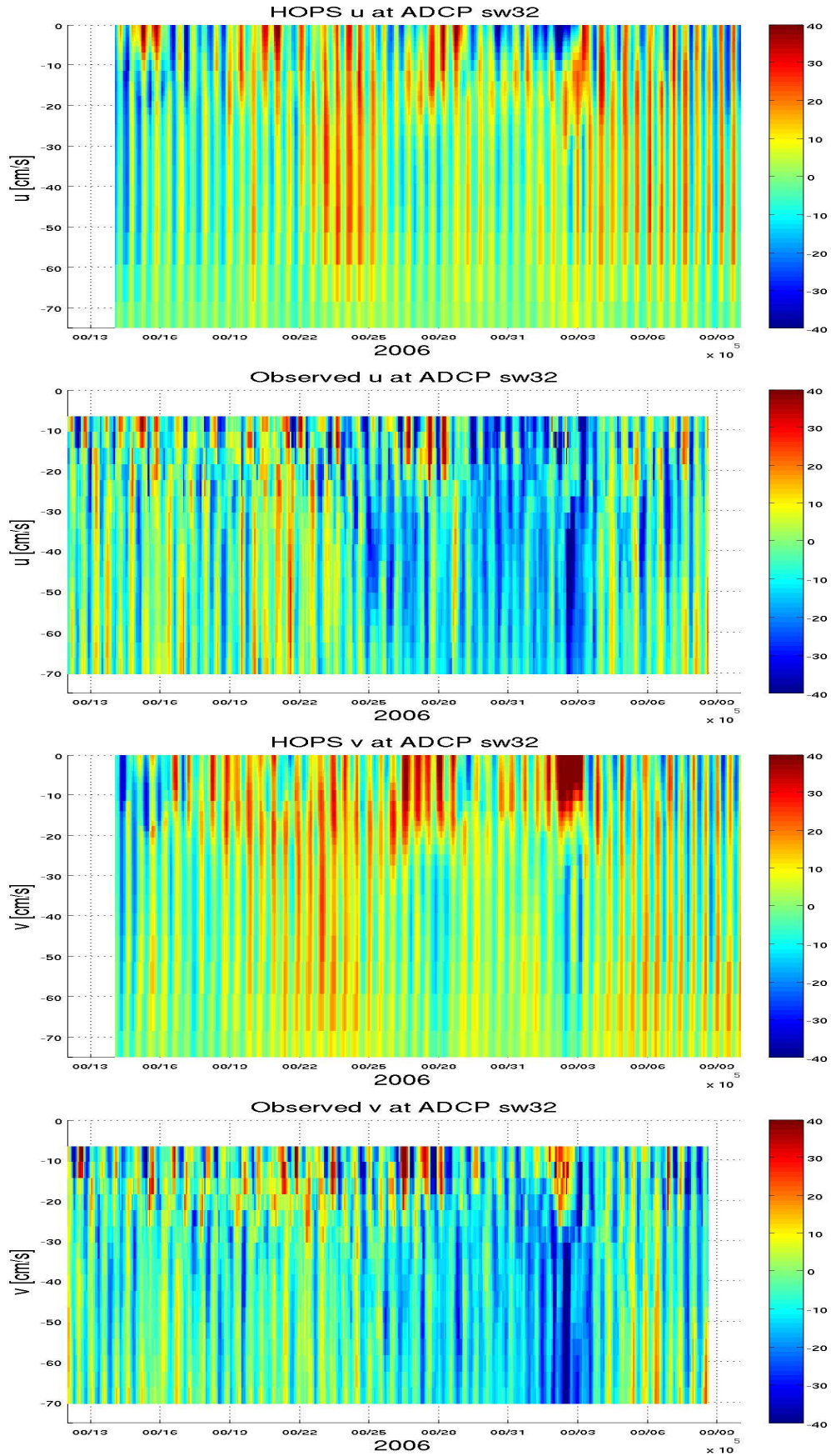
Figure 4. ADCP sw32, HOPS run in Jul10/PJH3/
