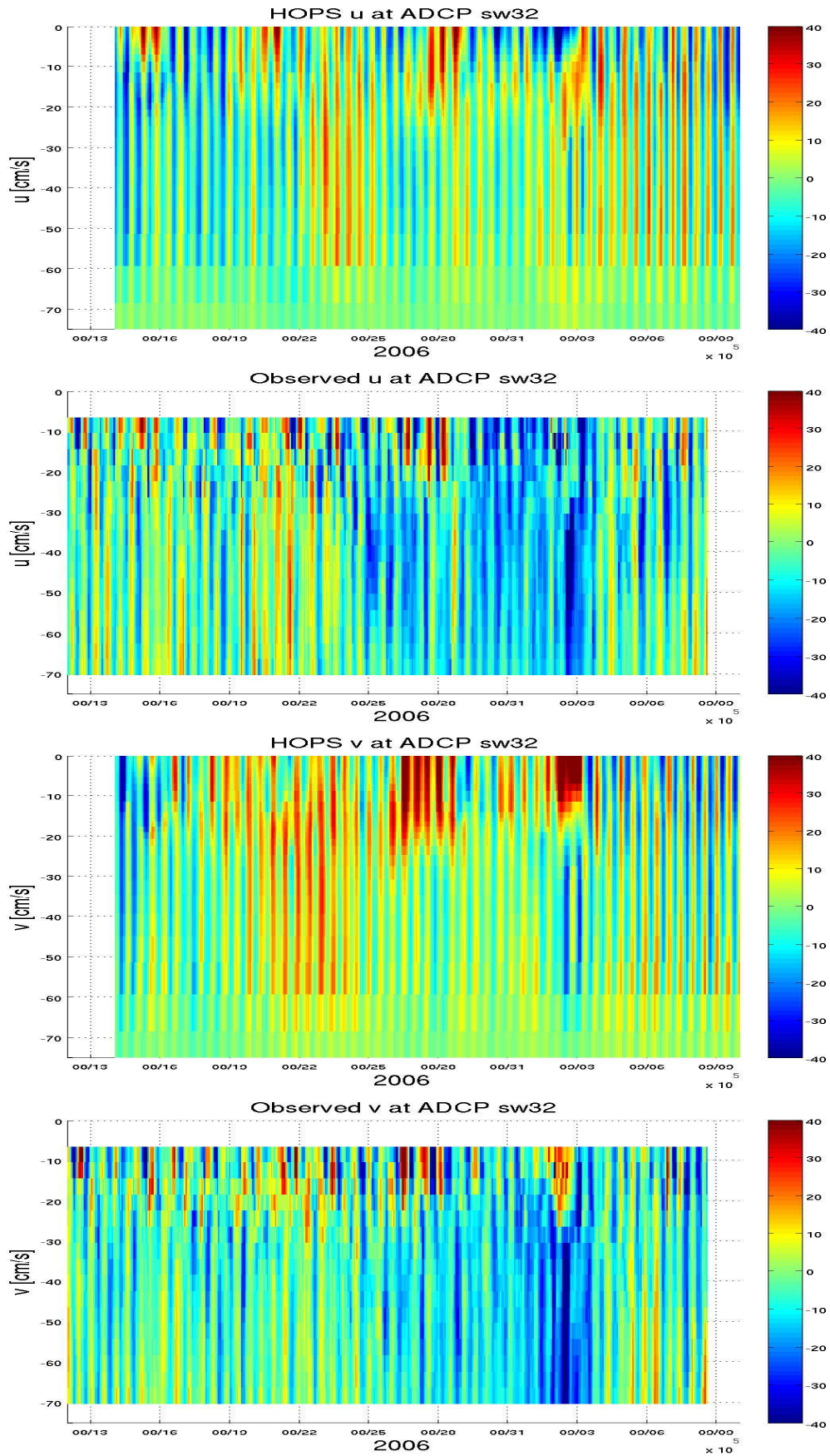
Figure 9. ADCP sw32, HOPS run in Jul10/PJH8/
