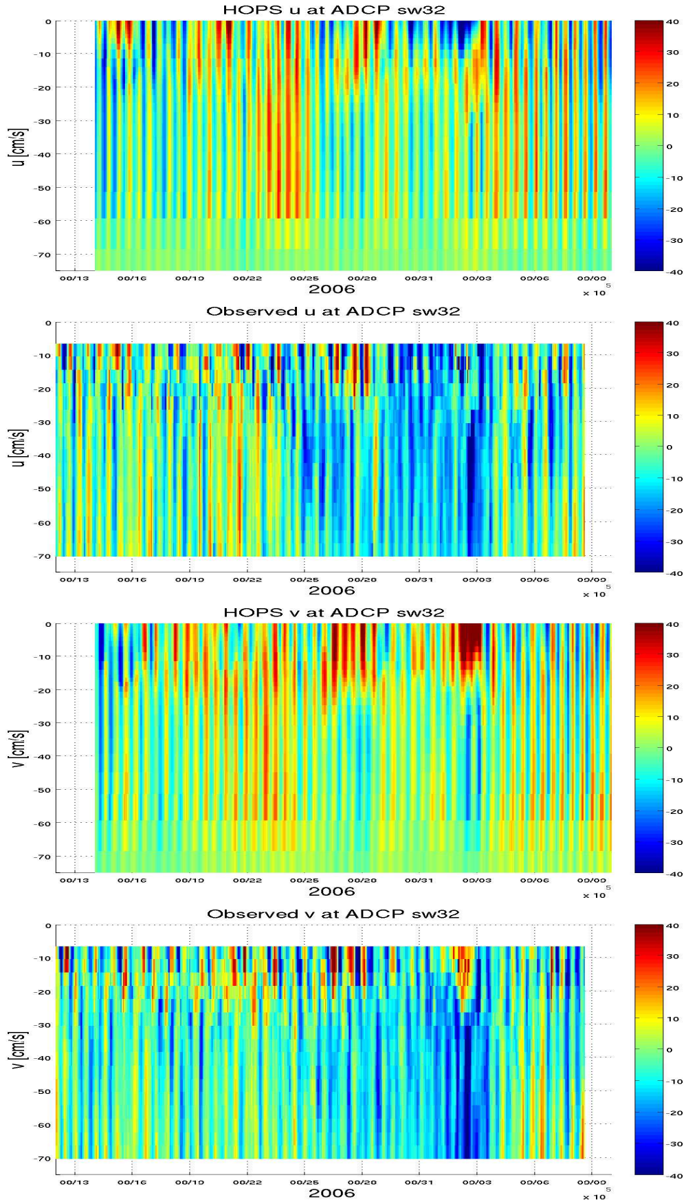
Figure 8. ADCP sw32, HOPS run in Jul10/PJH7/
