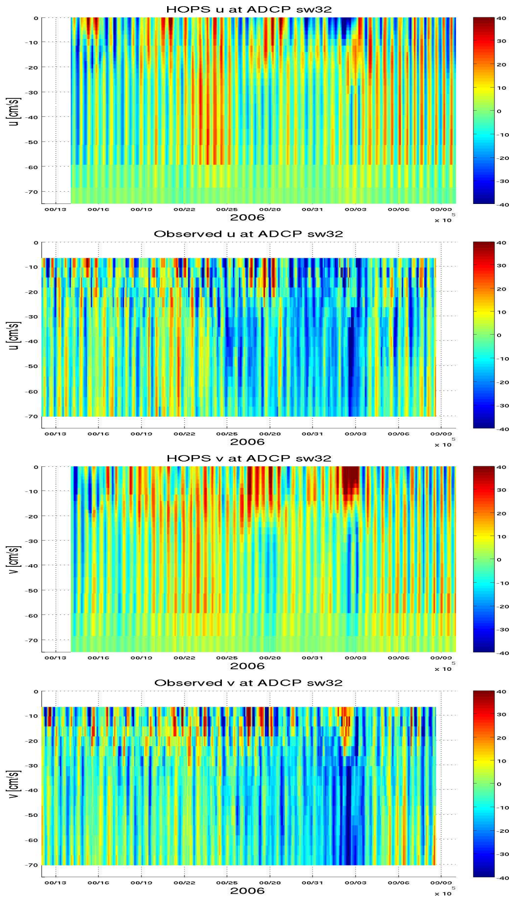
Figure 7. ADCP sw32, HOPS run in Jul10/PJH6/
