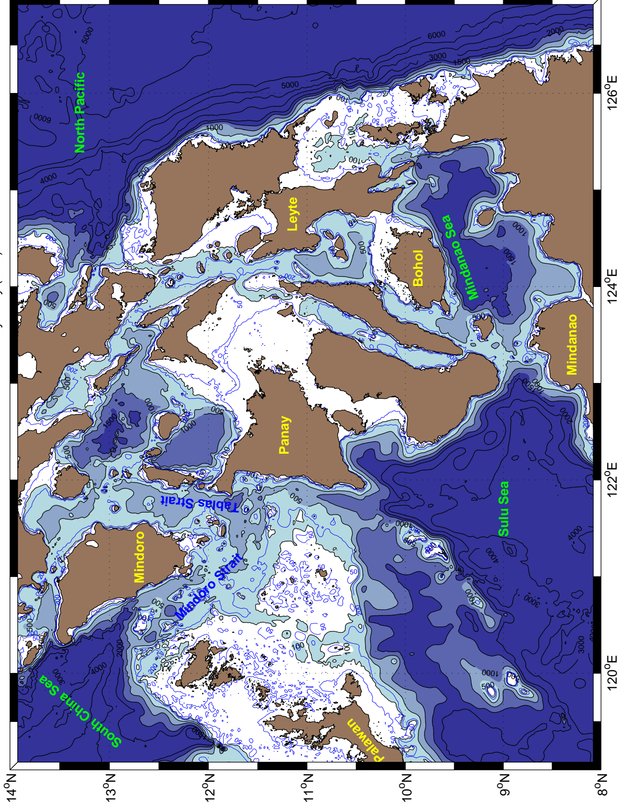
Smith and Sandwell 1-min Bathymetry (v9.1)
