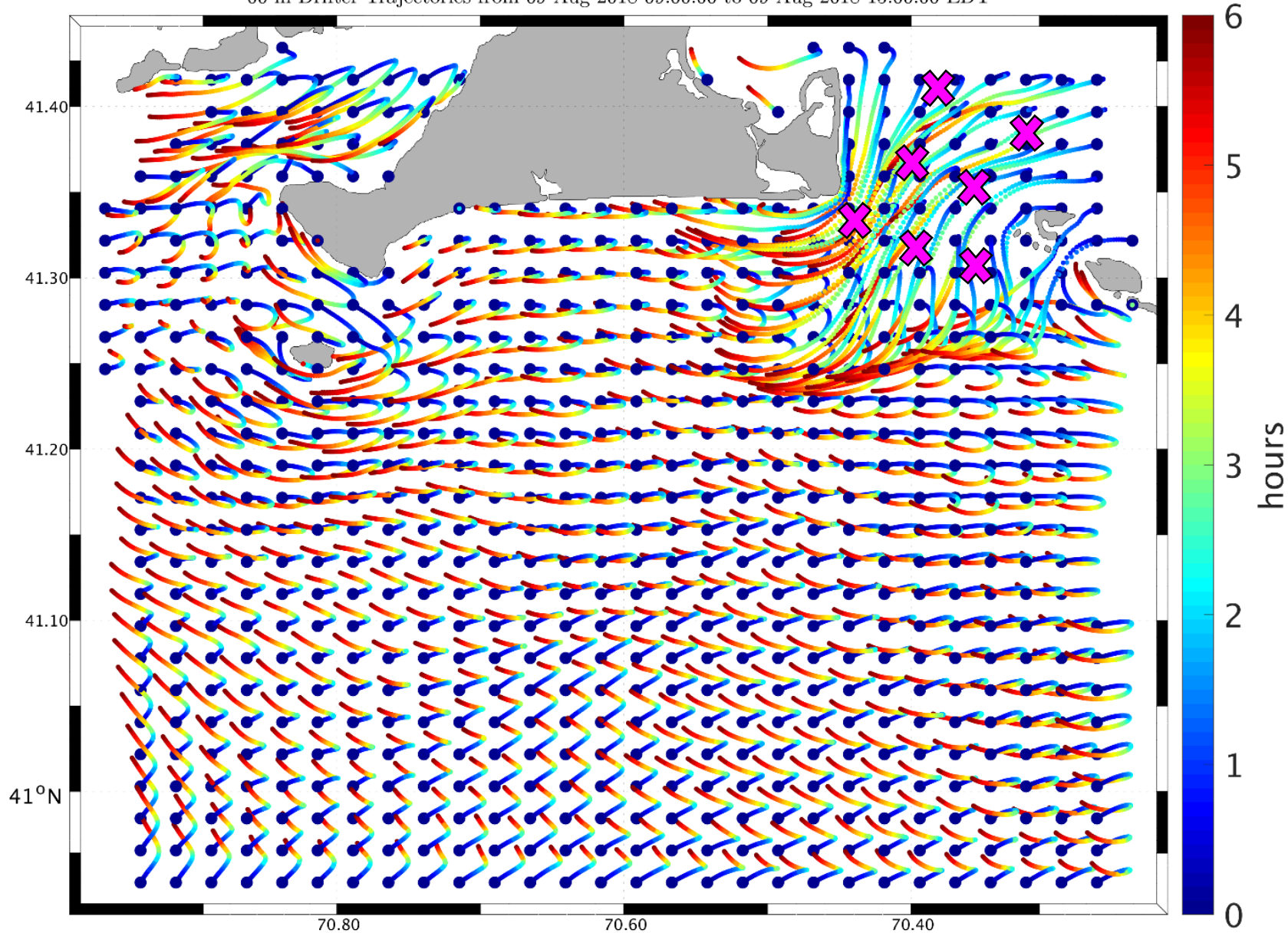
00 m Drifter Trajectories from 09-Aug-2018 09:00:00 to 09-Aug-2018 15:00:00 EDT
