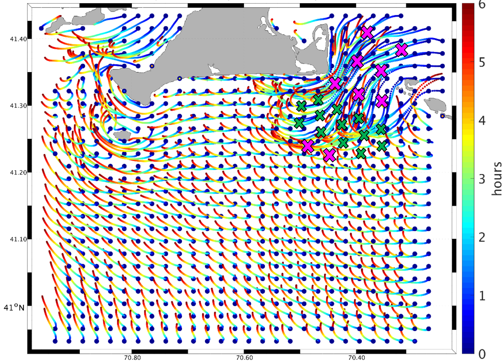
00 m Drifter Trajectories from 09-Aug-2018 11:00:00 to 09-Aug-2018 17:00:00 EDT
