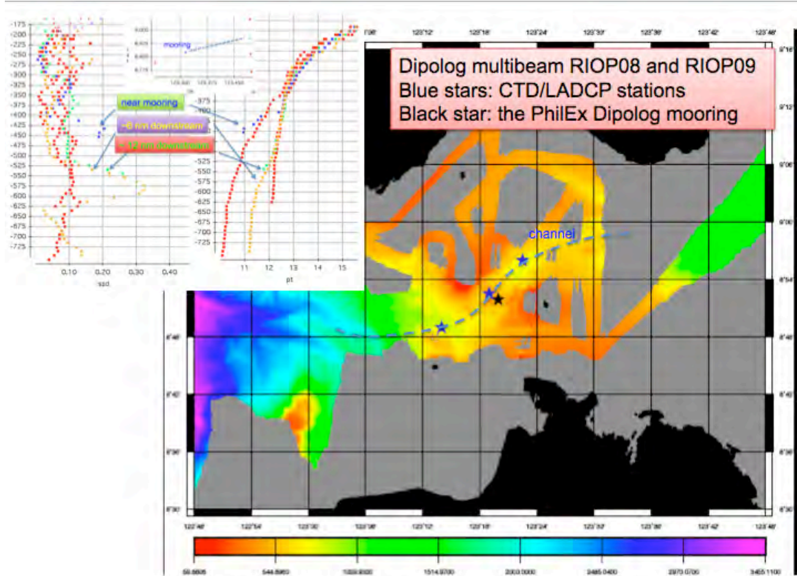
Figure 14 [added after figure sequence prepared]: Sea floor depths from RIOP08 and RIOP09 multibeam surveys. The blue stars mark the CTD/LADCP stations along the deep passage. The dashed blue line marks the approx channel axis. The black star is the position of the PhilEx Dipolog ADCP mooring, at 490 meters depth. The profiles of speed and temperature are shown in upper left panel. At the stations ~6 nm downstream of the moorings the speed maximum near 590 m is about 150 m above the sea floor, indicating that the overflow at least at times does not slide along the sea floor to great depths in the Mindanao Sea, perhaps a tidal effect?
