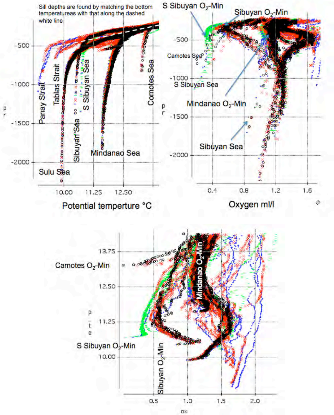
Figure 5: Potential Temperature and oxygen depth profiles in the interior seas of the Philippines [upper panel]; \theta/O_2 [lower panel]
