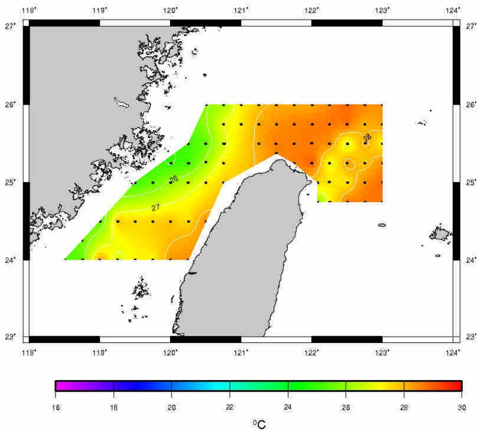
T at 10m depth, Aug 24-26, 2008
