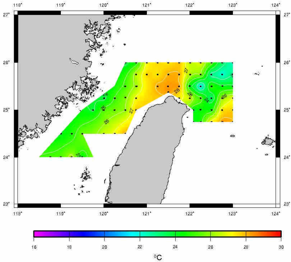
T at 50m depth, Aug 24-26, 2008
