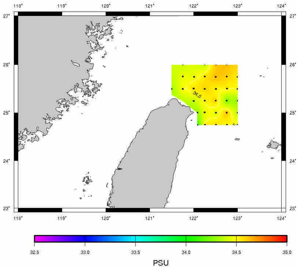
S at 100m depth, Aug 24-26, 2008
