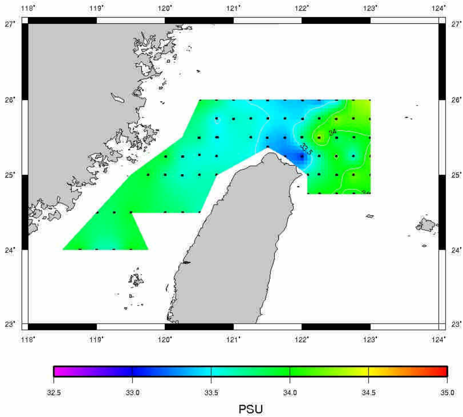
S at 50m depth, Aug 24-26, 2008
