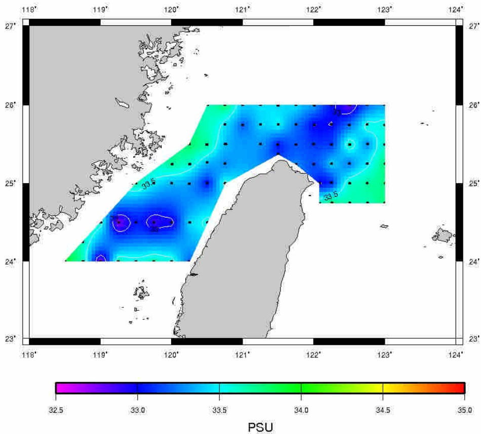
S at 10m depth, Aug 24-26, 2008
