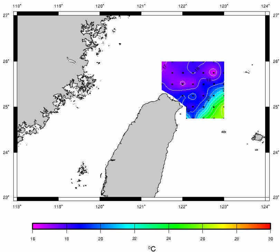
T at 100m depth, Aug 24-26, 2008
