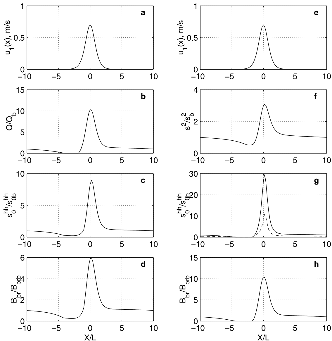
Figure 14. Model calculations of the sea surface manifestation of IW soliton (case 2 in Table 1). (a) Current velocity induced by IW on the sea surface. (b) Modulation of wave breaking. (c) Modulation of L-band NRCS at HH polarization. Solid line for total NRCS coincides with the line for Bragg scattering. Contribution of specular reflection and wave breaking is negligible. (d) Modulation of L-band Bragg wave spectrum. (e) Same as in Figure 14a. (f) Modulation of the mean square slope. (g) Modulation of X-band NRCS at HH polarization: solid line is total NRCS, and dashed line is sum of quasi-specular and wave breaking contributions. (h) Modulation of X-band Bragg wave spectrum. All quantities are normalized on the corresponding background value.
