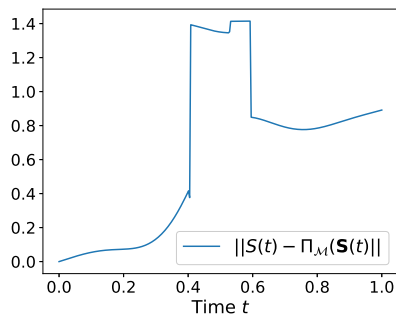
(b) Approximation error with respect to the exact reduction \Pi_{\mathcal{M}}(\mathbf{S}(t)) : i.e., \|\mathbf{S}(t) - \Pi_{\mathcal{M}}(\mathbf{S}(t))\| .
