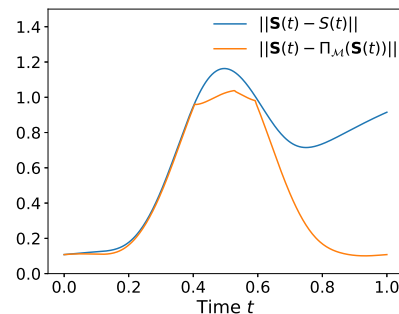
(c) Errors with respect to the full \mathbf{S}(t) : dynamical error (blue) vs. best achievable error (orange).
