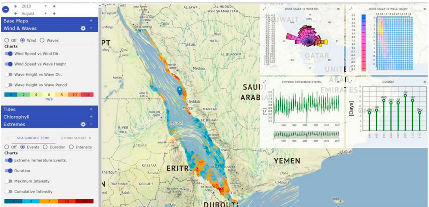
Fig. 8. The RedSeaAtlas system showing overall wind patterns and statistics (at the dropped pin location, here north of Jeddah in the central Red Sea) of extreme temperature events in the Red Sea. Users can select any region to show more detailed information and associated attributes through different charts (Afzal et al. 2019b).
