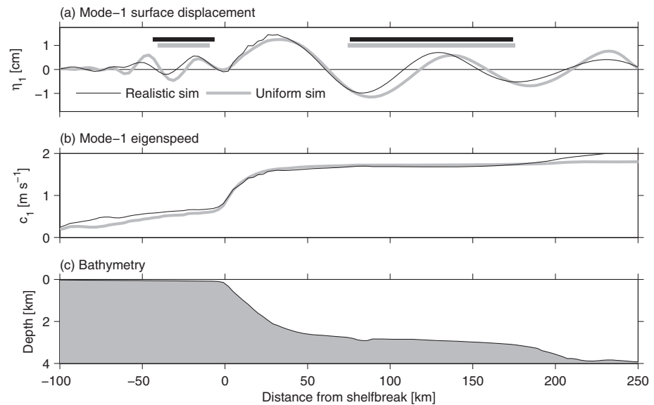
Figure 8. Across-slope snapshots at 02:48 1 September 2016 of mode-1 surface displacement indicate different wavelengths in the realistic (black) and uniform (gray) MSEAS primitive-equation simulations. (b) The simulated wavelengths agree with theoretical wavelengths (bars) determined from 42 day average eigenspeeds. The bathymetry is shown in Figure 8c.
