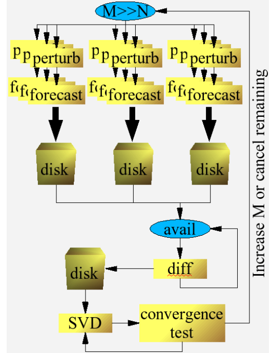
Figure 4: The parallel ESSE implementation
