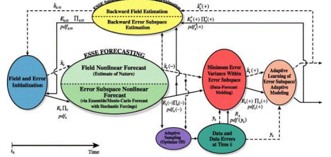
Figure 2: The ESSE algorithm
