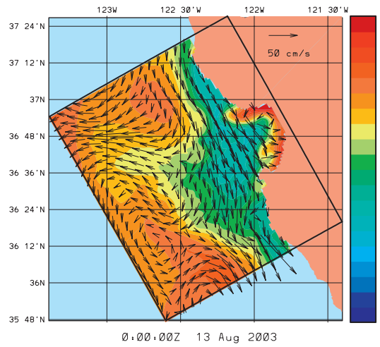
Fig. 7. Comparisons of (top row) available real-time SST ( ^{\circ}\text{C} ) images from satellite (August 12 and 21) and aircraft (August 13) with (bottom row) corresponding real-time forecast surface temperature ( ^{\circ}\text{C} ) fields. Note timing conventions (e.g. 0000Z August 13 forecast corresponds to 1600 local August 12 and is compared to August 12 image).
