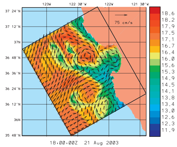
Fig. 7. Comparisons of (top row) available real-time SST ( ^{\circ}\text{C} ) images from satellite (August 12 and 21) and aircraft (August 13) with (bottom row) corresponding real-time forecast surface temperature ( ^{\circ}\text{C} ) fields. Note timing conventions (e.g. 0000Z August 13 forecast corresponds to 1600 local August 12 and is compared to August 12 image).
