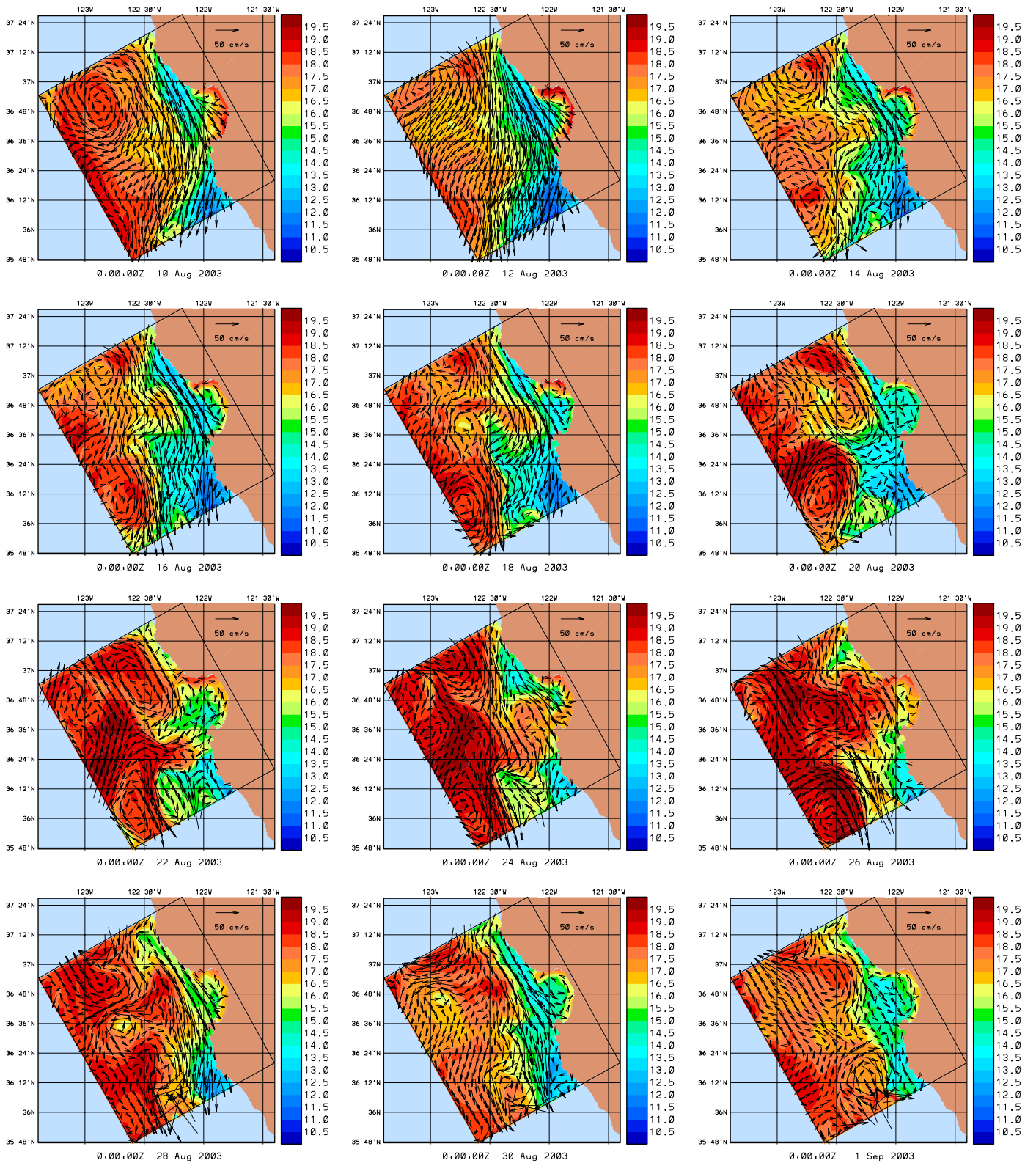
Fig. 13. Reanalysis surface temperature (°C) and velocity (cm/s) every two days for the period August 10–September 1, 2003.
