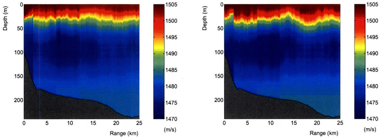
(a) Principal estimation of water column SVP
