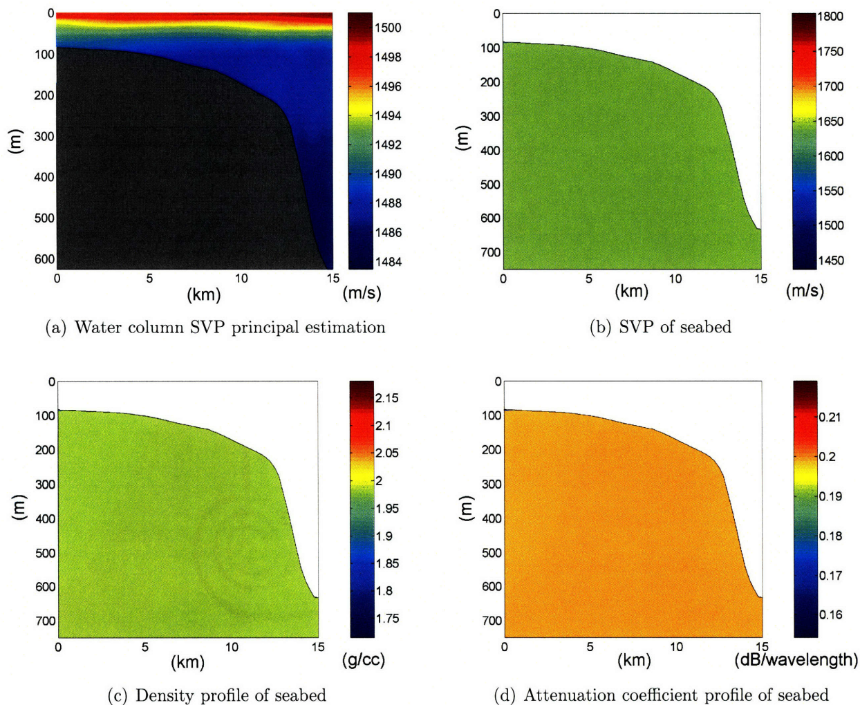
Figure 9-8: Bearing 7, Aug. 25, 2006.
