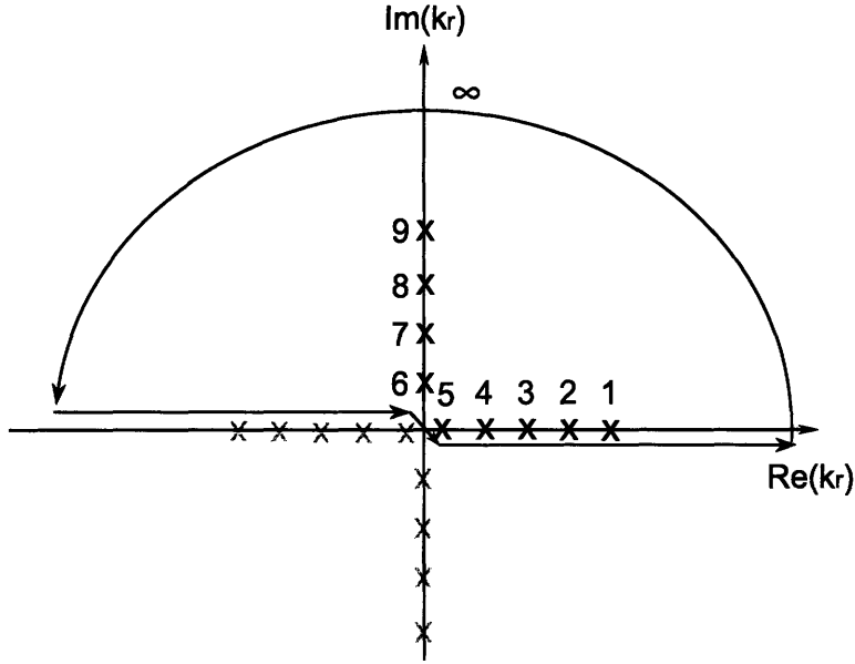
Figure C-1: Idea waveguide
