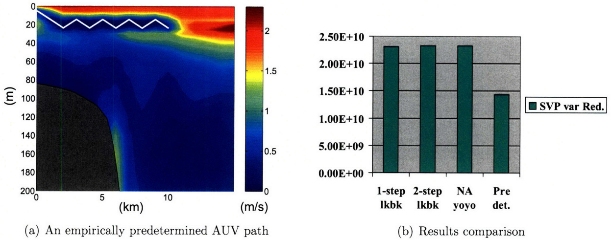
Figure 9-13: Aug. 21, 2006, bearing 5, AUV path planning for capturing SVP prediction uncertainty. Lr = 1000m, Lz = 5m . 1-step look-back: 2.30776e+10 , 2-step look-back: 2.32952e+10 , non-adaptive yoyo: 2.32836e+10 , predetermined: 1.43376e+10 . The unit is (m/s)^2 \cdot m^2 .
