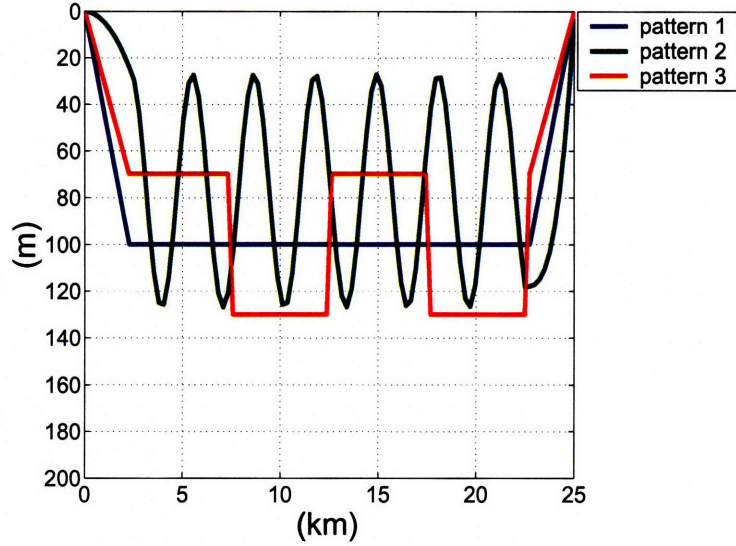
Figure 6-2: Illustration of 3 yoyo patterns.
