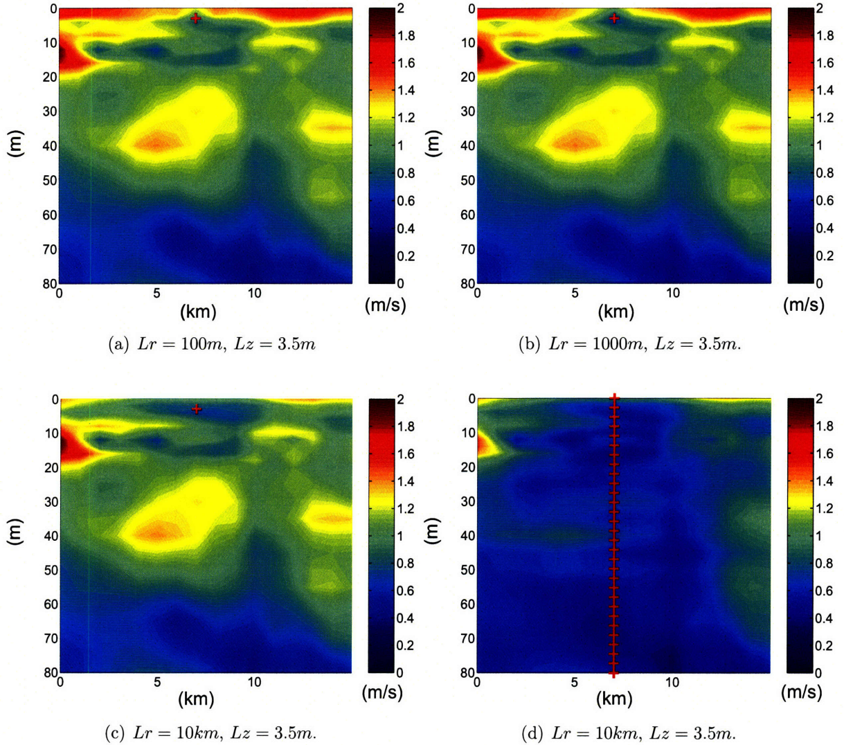
Figure 7-9: The posterior SVP prediction error standard deviation. In (a), (b) and (c), an in-situ measurement is made at (7km, 3m) . In (d), 30 in-situ measurements are made at the range of 7km .
