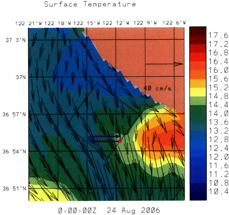
Figure 8-1: Illustration of a front prediction from HOPS/ESSE and a predetermined AUV path for capturing the front.
