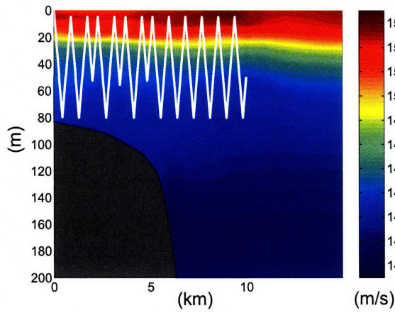
(a) p = 40, \gamma = 0.5 , posterior SVP prediction
