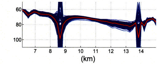
(c) Multiplier=0.8, Receiver Depth=165m
