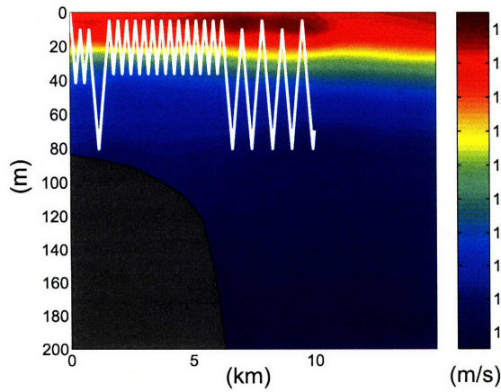
(e) p = 20, \gamma = 0.5 , posterior SVP prediction
