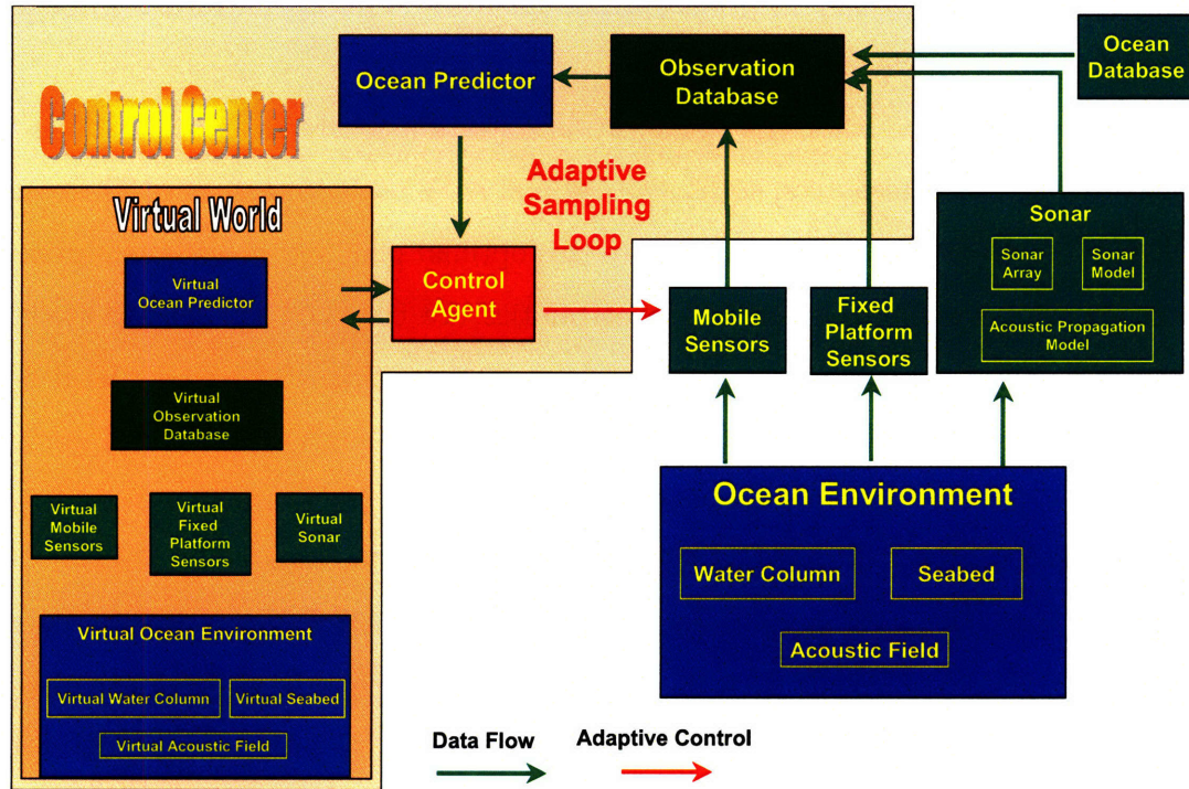
Figure 3-5: AREA wiring diagram from an operational viewpoint.
