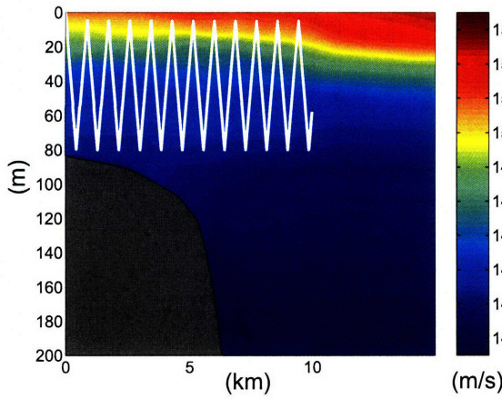
(c) p = 20, \gamma = 0.9 , posterior SVP prediction
