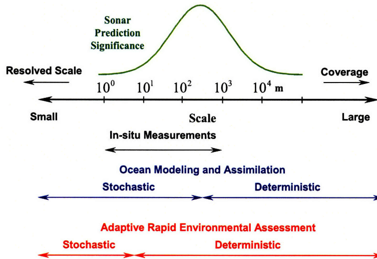
Figure 3-1: Multi-scale environmental assessment. The typical sonar systems performance is dependent on acoustic environment variability over a wide range of scales. Optimal environmental assessment will therefore be a compromise between conflicting requirements of coverage and resolution. By targeting areas of high sensitivity to the sonar system through in situ measurements, the deterministic assessment range will be shifted towards smaller scales.
