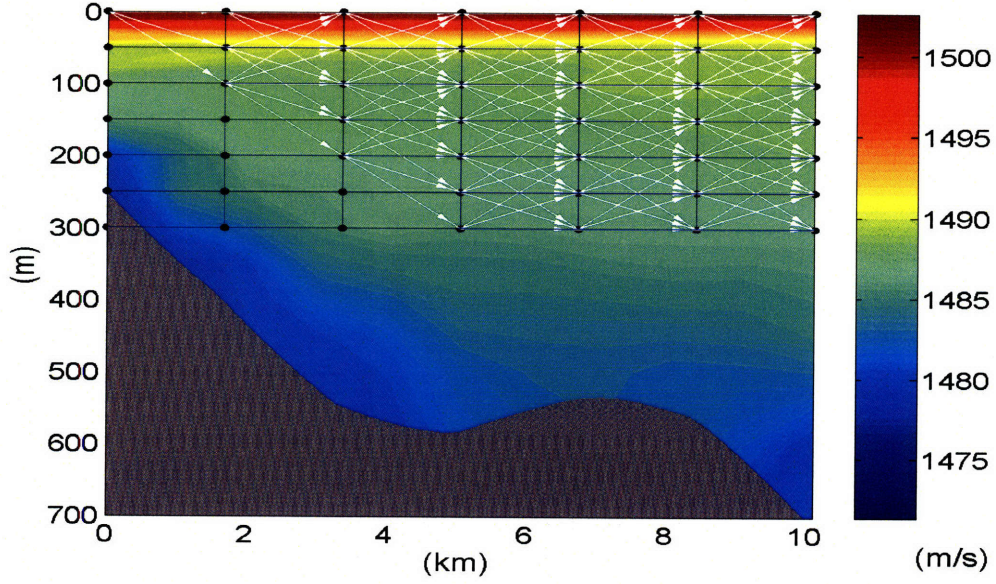
Figure 5-3: Illustration of ocean discretization for AUV path.
