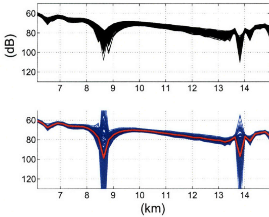
(b) L_r = 25m, L_z = 0.1m , Receiver Depth=165m
