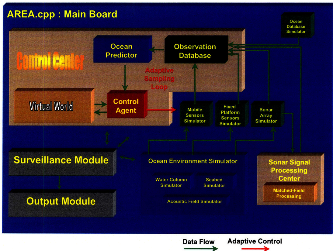
Figure 7-1: AREA simulation framework wiring diagram
