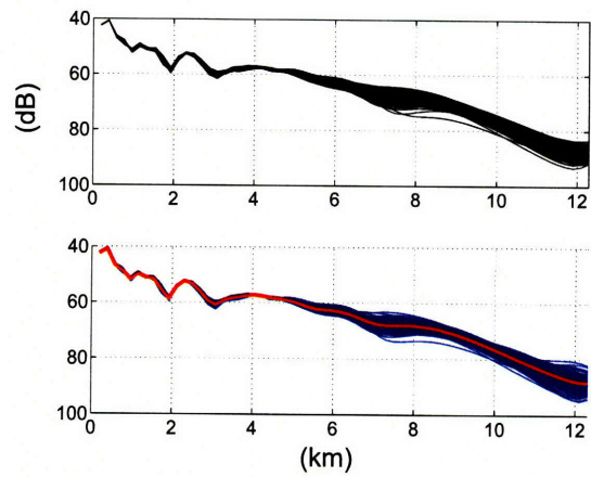
(b) TLs comparison at the depth of 75m
