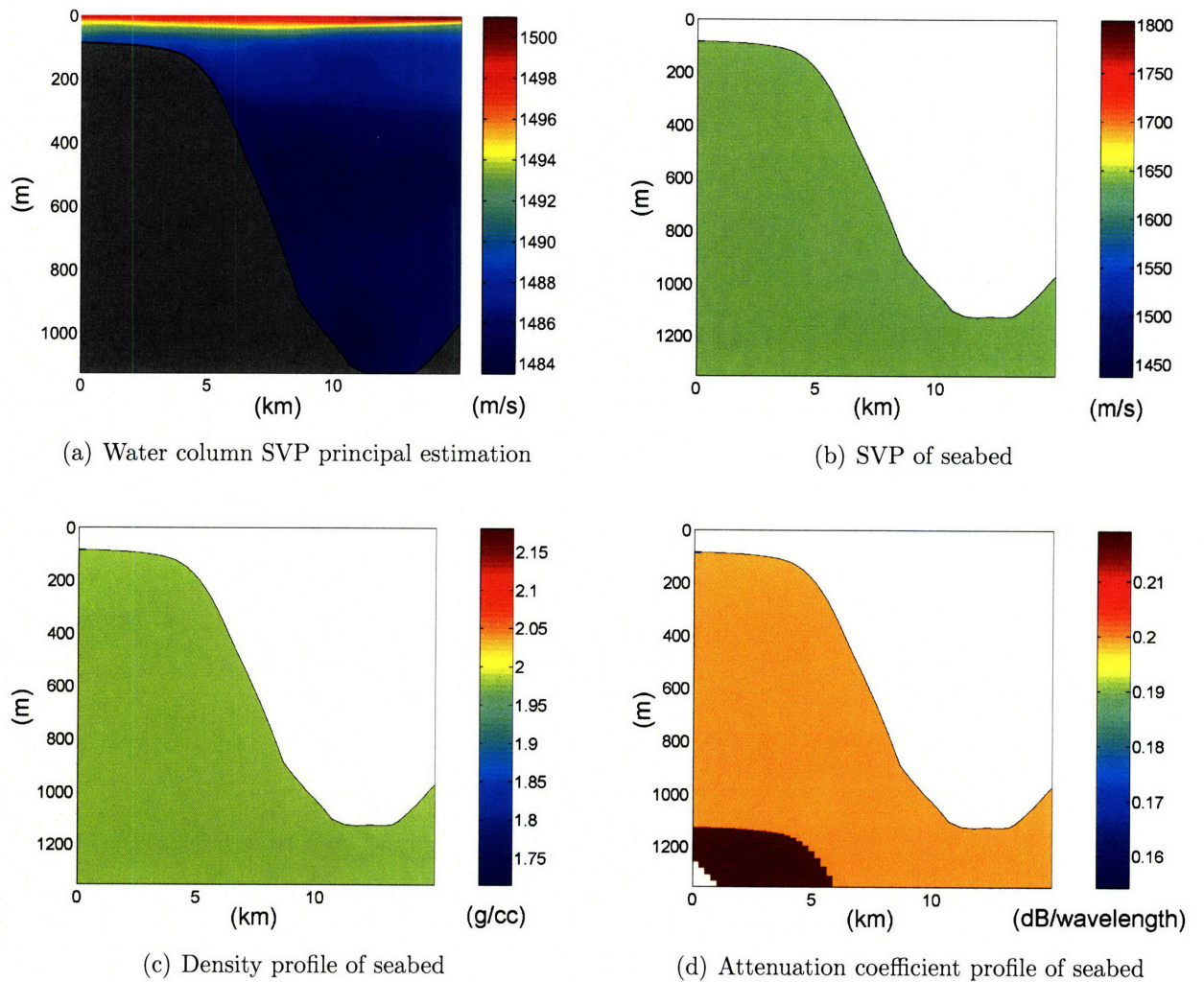
Figure 9-7: Bearing 6, Aug. 25, 2006.
