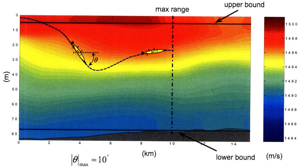
Figure 5-1: Illustration of constraints on the AUV path.
