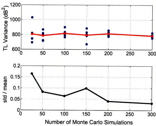
(c) Convergence test of Monte Carlo simulations
